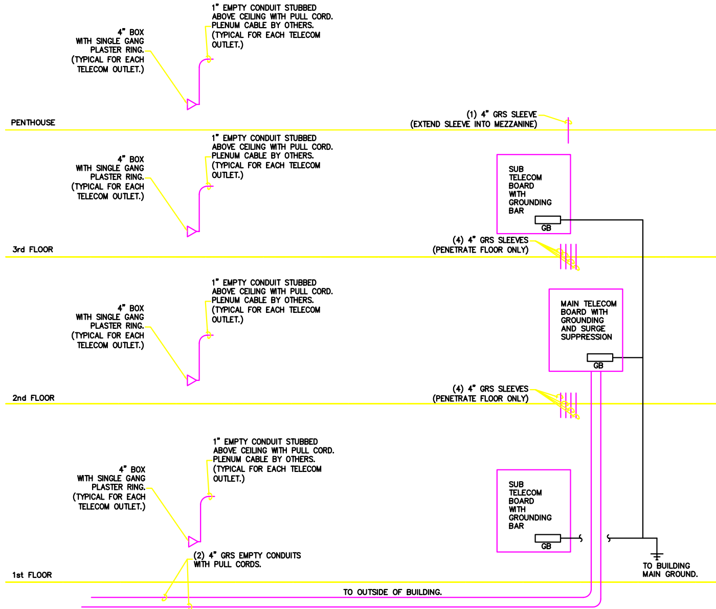
Telcom Riser Diagram
